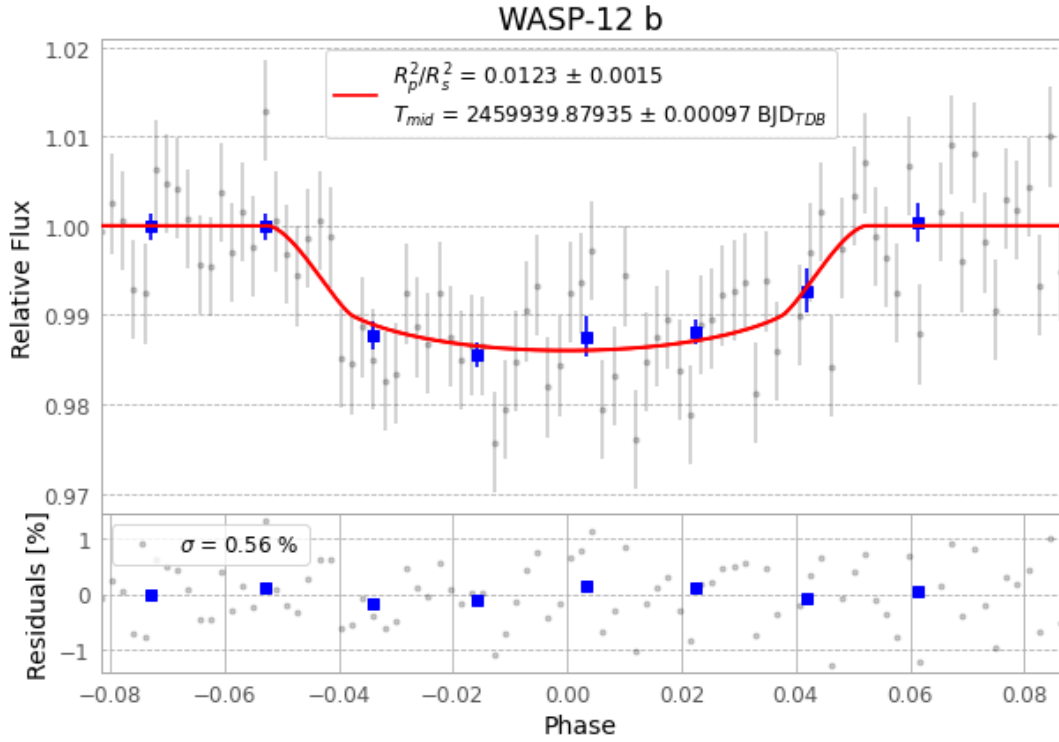
Figure 1 — FinalLightCurve_WASP-12 b_2022-12-25.png (SHA-256 efb8494999849d88...)
