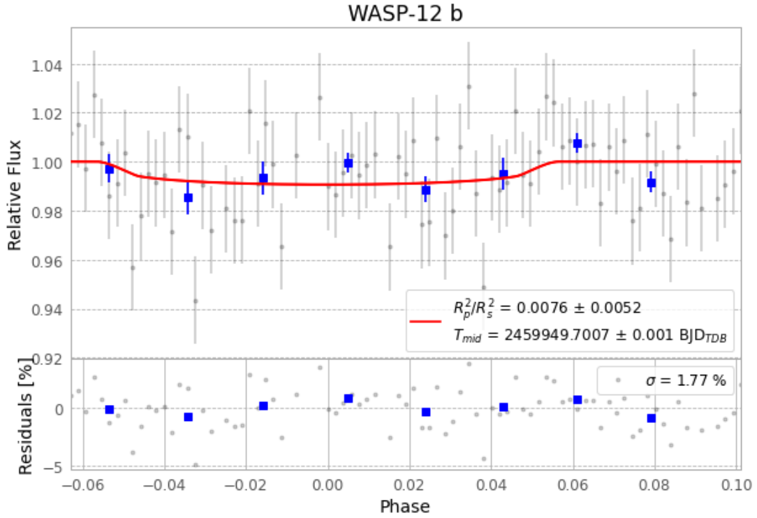
Figure 1 — FinalLightCurve_WASP-12 b_2023-01-04.png (SHA-256 a6798523faa477b2...)
