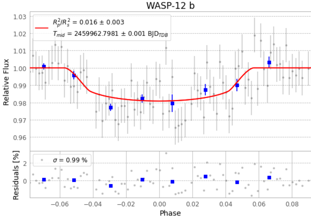
Figure 1 — FinalLightCurve_WASP-12 b_2023-01-17.png (SHA-256 893fa5629be1c948...)
