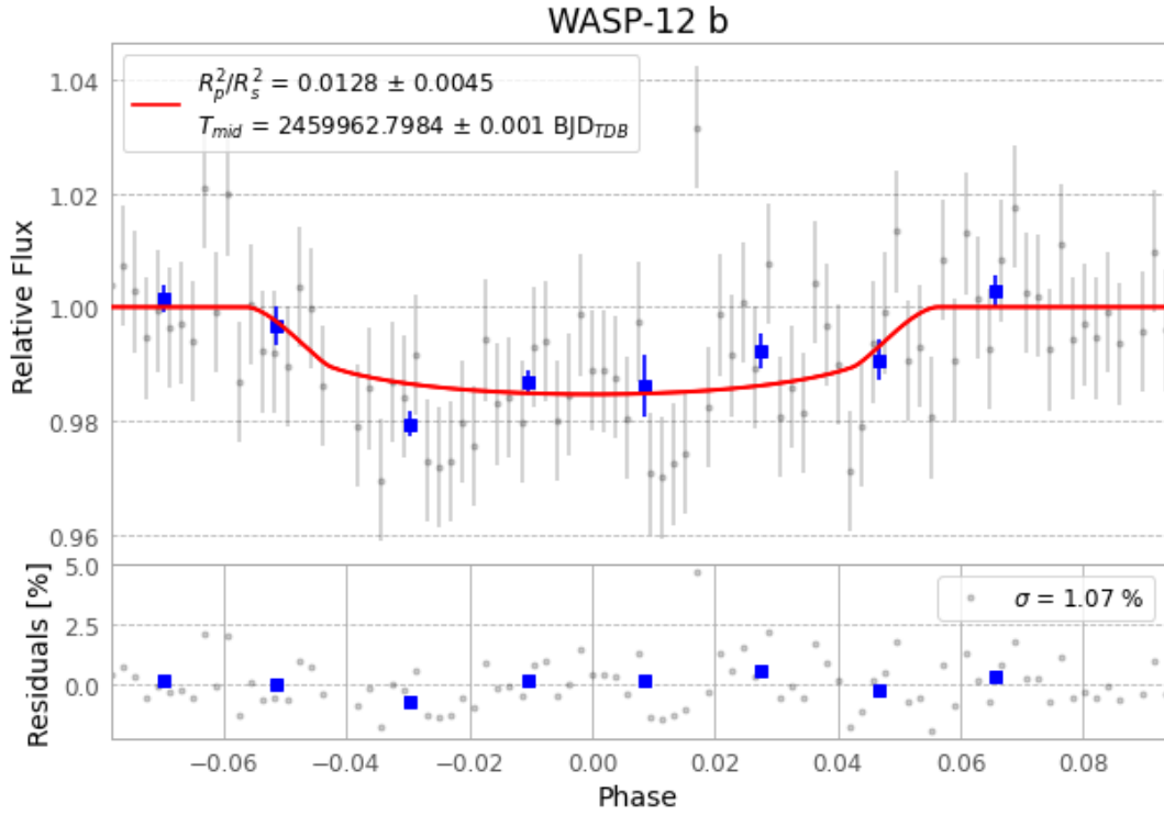
Figure 1 — FinalLightCurve_WASP-12 b_2023-01-17.png (SHA-256 9c5b9310900589d1...)
