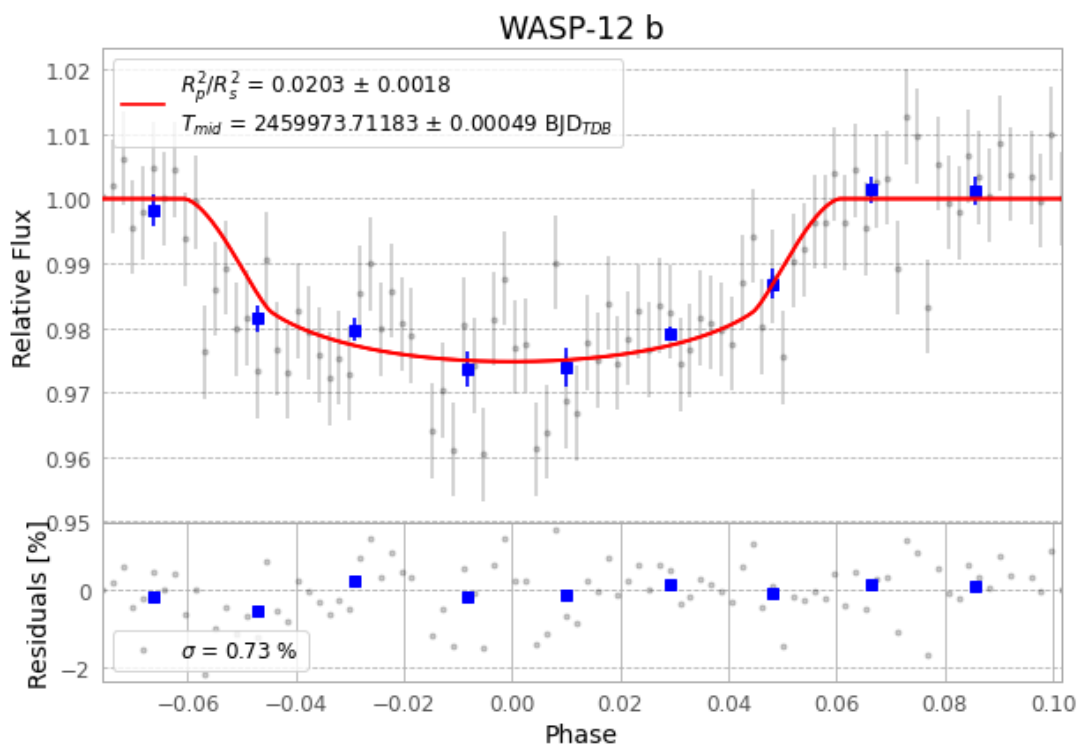
Figure 1 — FinalLightCurve_WASP-12 b_2023-01-28.png (SHA-256 53c76f64822473ac...)
