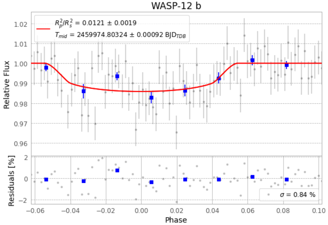
Figure 1 — FinalLightCurve_WASP-12 b_2023-01-29.png (SHA-256 68decd16359a6763...)
