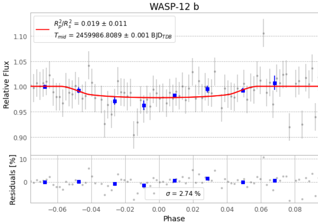
Figure 1 — FinalLightCurve_WASP-12 b_2023-02-10.png (SHA-256 9a76e6380c37e523...)
