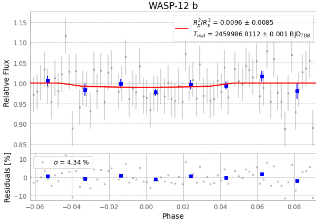
Figure 1 — FinalLightCurve_WASP-12 b_2023-02-10.png (SHA-256 8d9dd1d4d20c54e4...)
