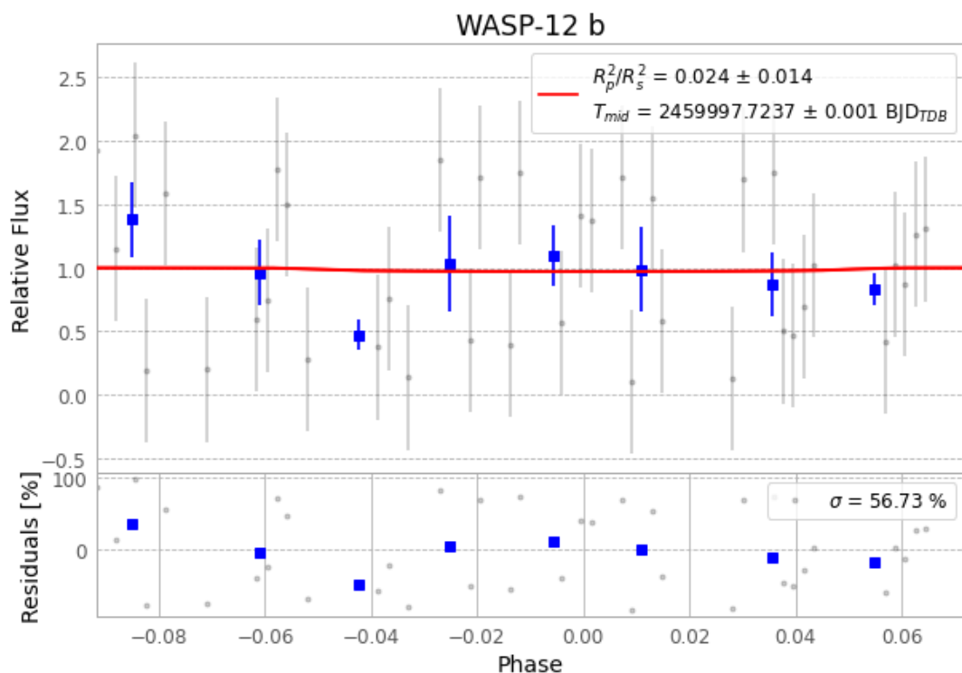
Figure 1 — FinalLightCurve_WASP-12 b_2023-02-21.png (SHA-256 3ff869e5d573b37a...)
