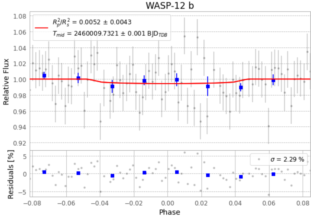
Figure 1 — FinalLightCurve_WASP-12 b_2023-03-05.png (SHA-256 ae62c6ec8fa4c0dc...)
