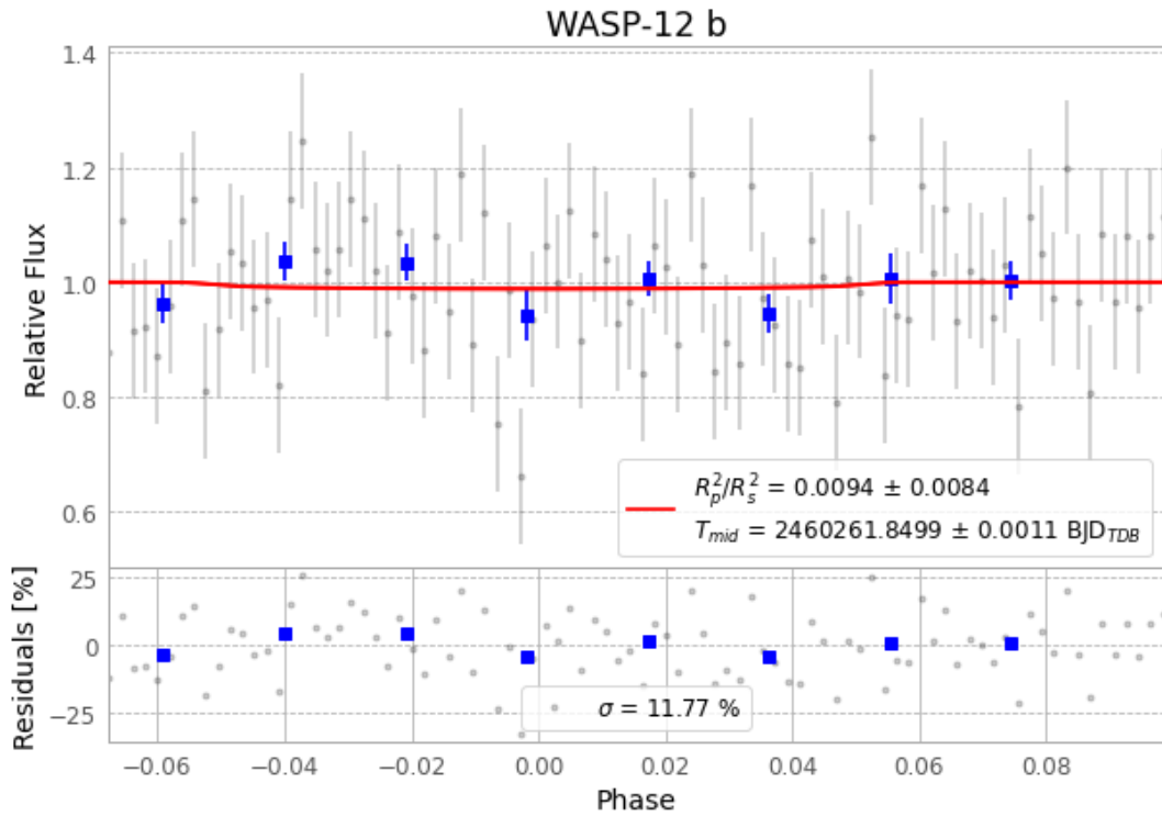
Figure 1 — FinalLightCurve_WASP-12 b_2023-11-12.png (SHA-256 ca7a9694213c9af1...)
