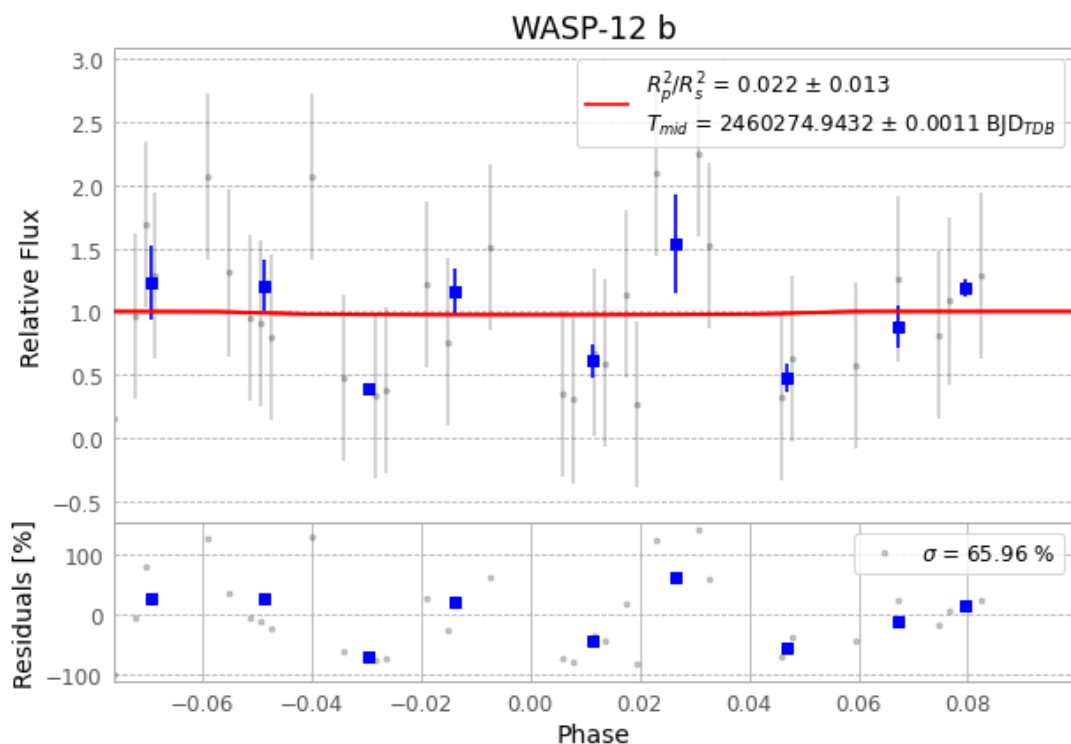
Figure 1 — FinalLightCurve_WASP-12 b_2023-11-26.png (SHA-256 bb13a87cceb64a75...)
