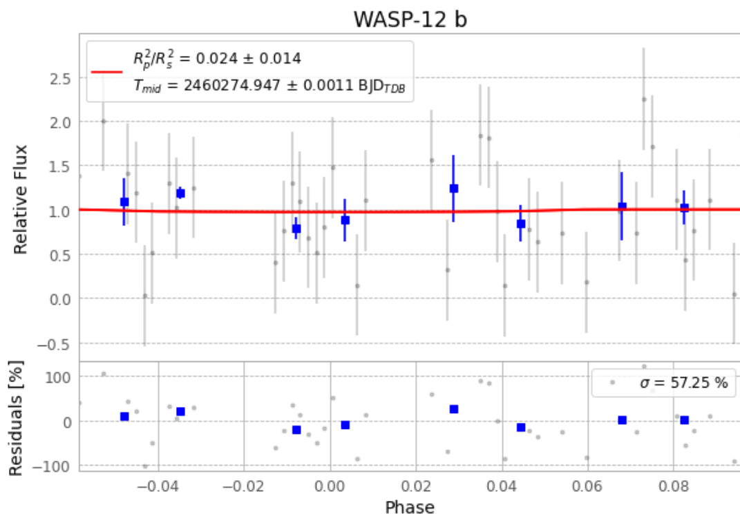
Figure 1 — FinalLightCurve_WASP-12 b_2023-11-26.png (SHA-256 0482d6fc8e35fccf...)
