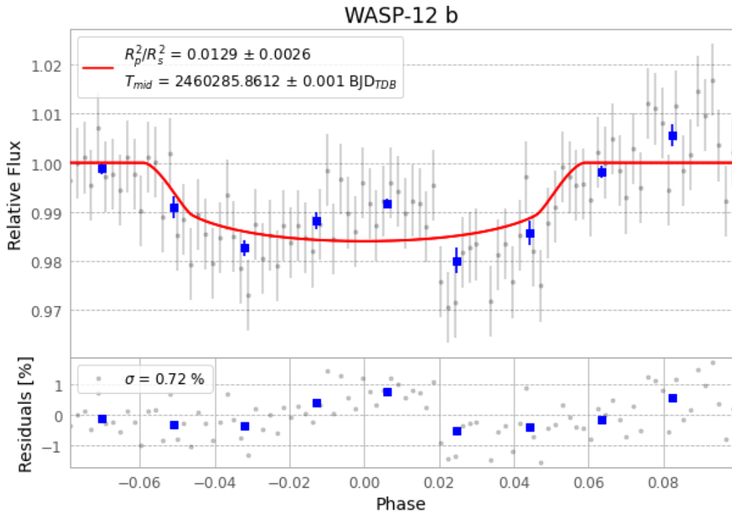
Figure 1 — FinalLightCurve_WASP-12 b_2023-12-06.png (SHA-256 cceb62b9eb270dbd...)
