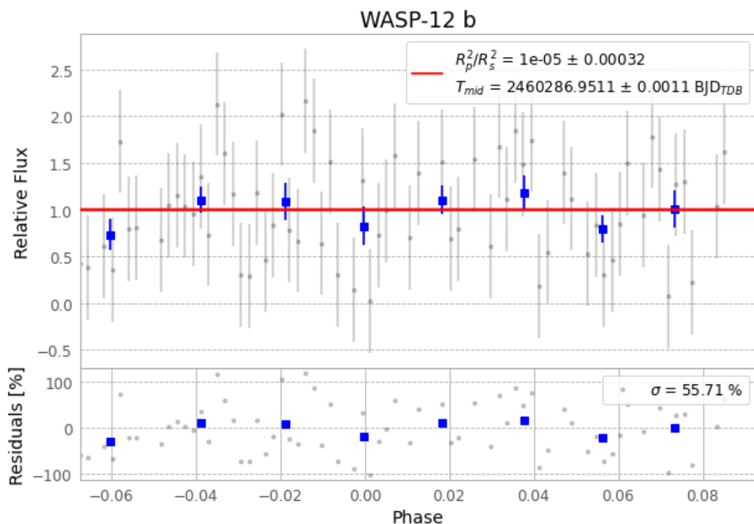
Figure 1 — FinalLightCurve_WASP-12 b_2023-12-08.png (SHA-256 60dbac18caa5611e...)
