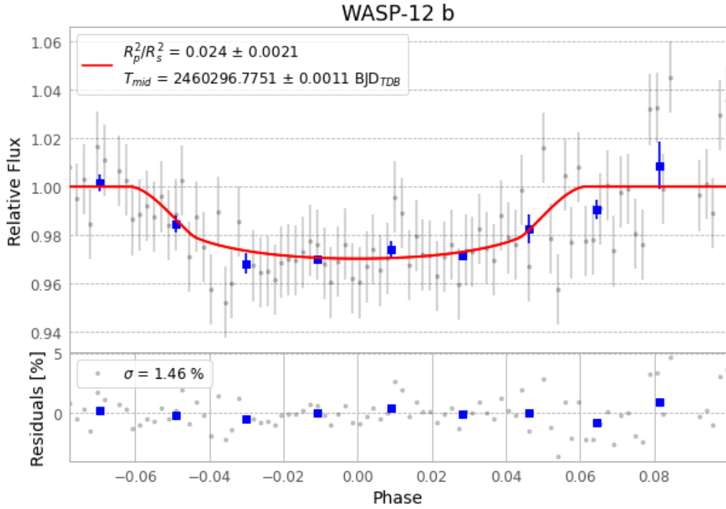
Figure 1 — FinalLightCurve_WASP-12 b_2023-12-17.png (SHA-256 671ad40ec44baf86...)
