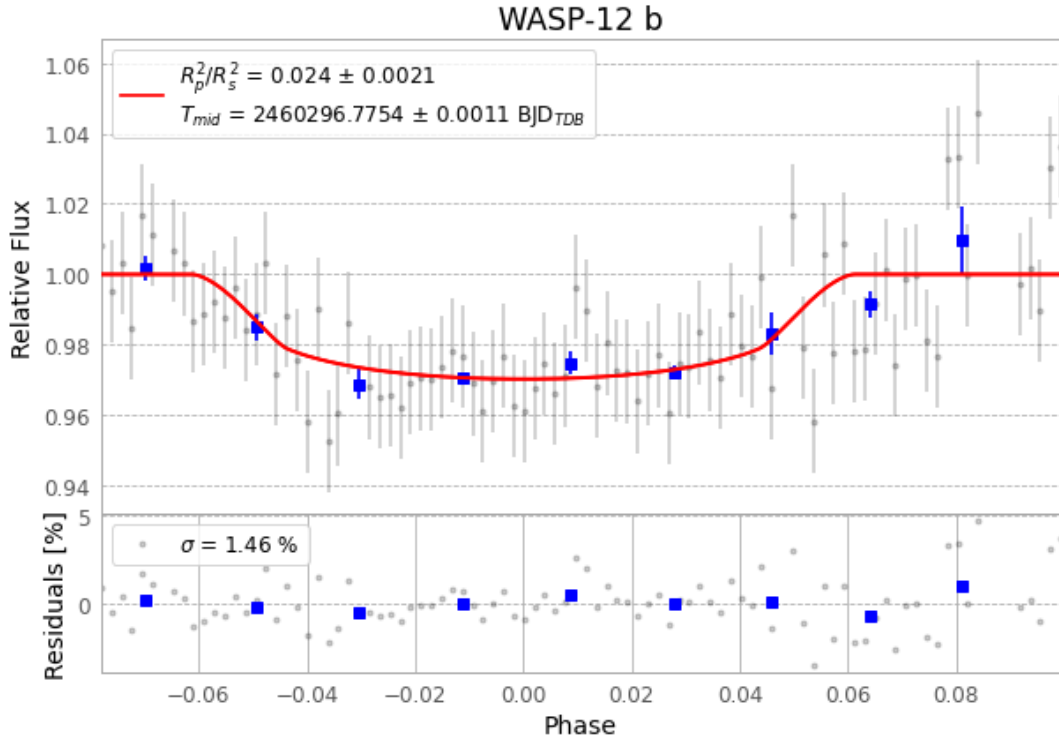
Figure 1 — FinalLightCurve_WASP-12 b_2023-12-17.png (SHA-256 d14f2e319c93d4e6...)
