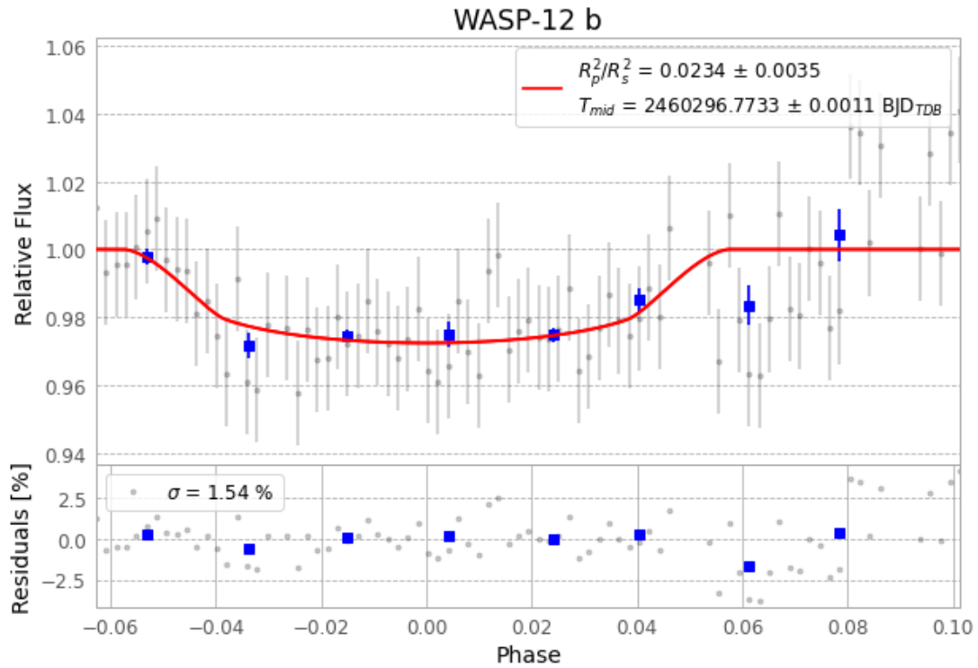
Figure 1 — FinalLightCurve_WASP-12 b_2023-12-17.png (SHA-256 3431716c1f66cd27...)
