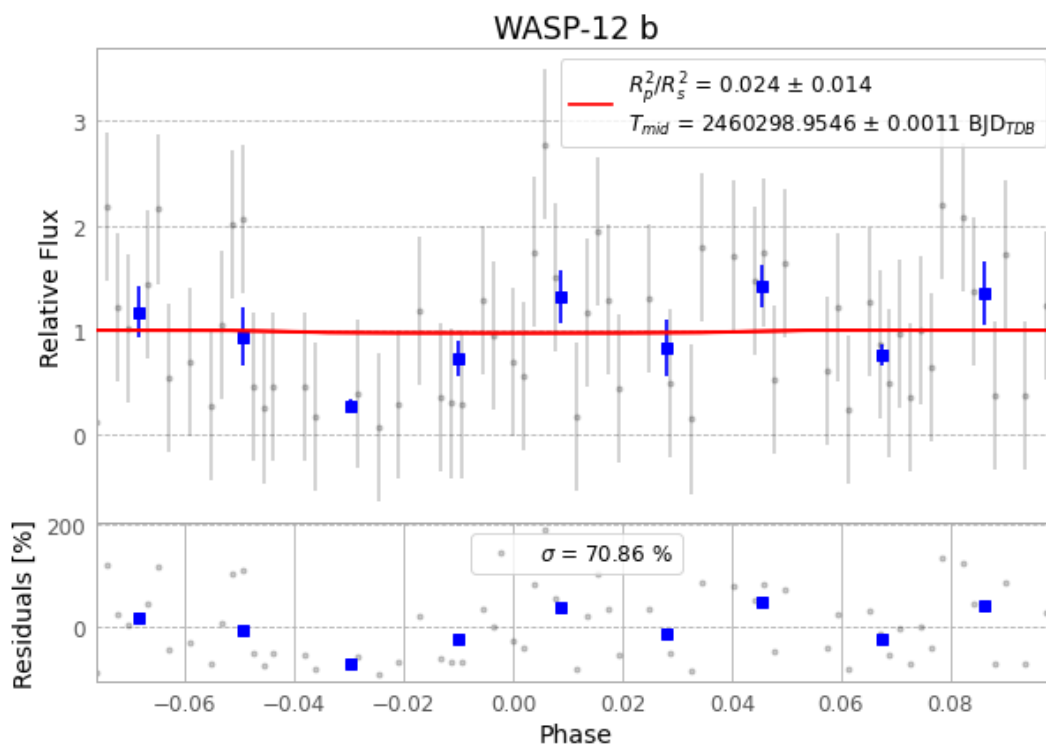
Figure 1 — FinalLightCurve_WASP-12 b_2023-12-20.png (SHA-256 d46b7214bd096146...)
