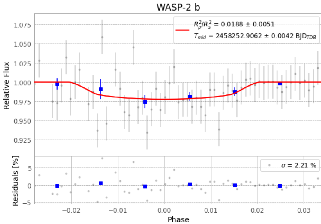
Figure 1 — FinalLightCurve_WASP-2 b_2018-05-14.png (SHA-256 25be0be95f163bde...)
