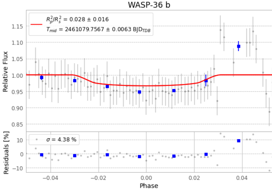
Figure 1 — FinalLightCurve_WASP-36 b_2026-02-07.png (SHA-256 f69b4a24660d27c4...)
