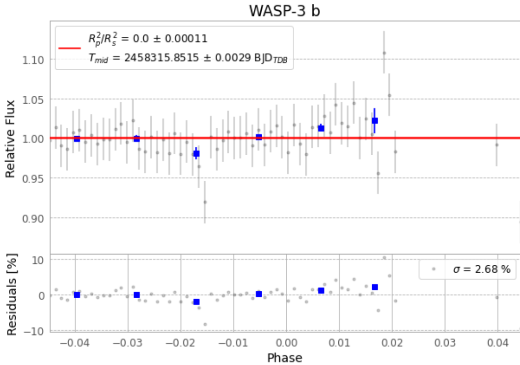
Figure 1 — FinalLightCurve_WASP-3 b_2018-07-15.png (SHA-256 f6dc64af8ca3b09c...)
