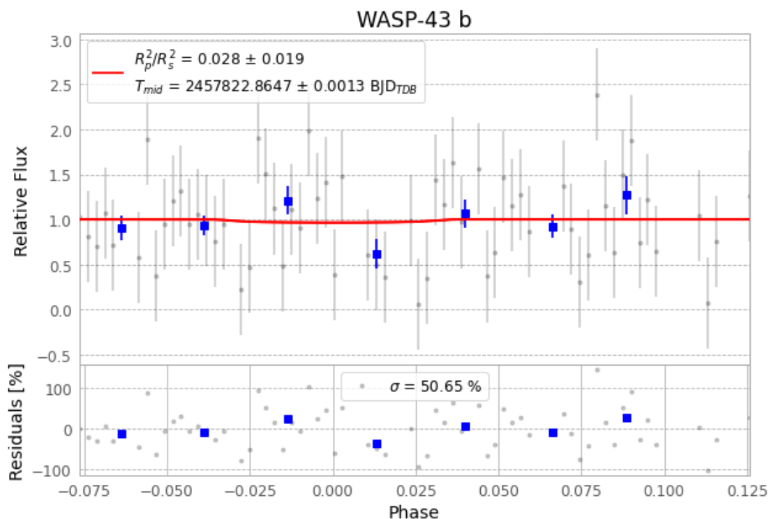
Figure 1 — FinalLightCurve_WASP-43 b_2017-03-10.png (SHA-256 2739a117129af632...)
