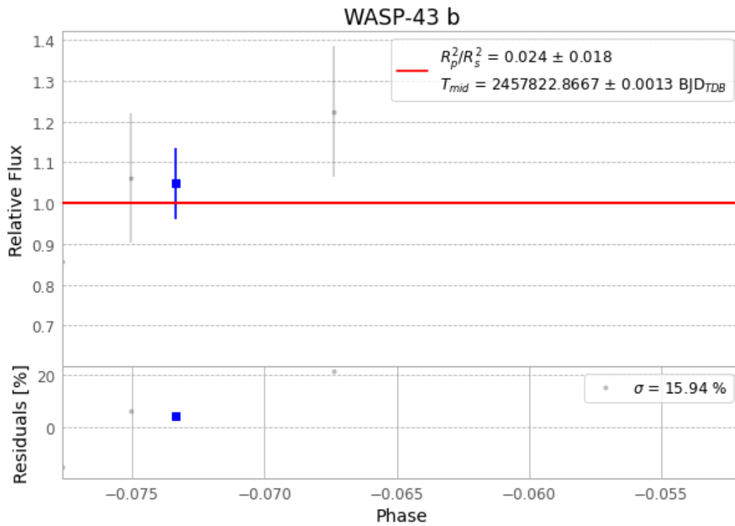
Figure 1 — FinalLightCurve_WASP-43 b_2017-03-10.png (SHA-256 64941f43a23f8f91...)
