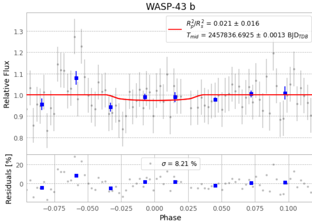
Figure 1 — FinalLightCurve_WASP-43 b_2017-03-23.png (SHA-256 dd9dad9f71bbf3e...)
