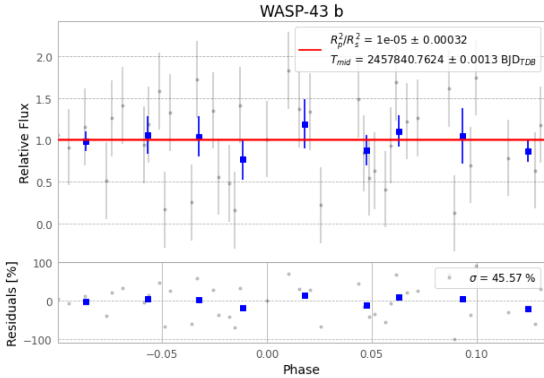
Figure 1 — FinalLightCurve_WASP-43 b_2017-03-27.png (SHA-256 6d80870b8f3e3b88...)
