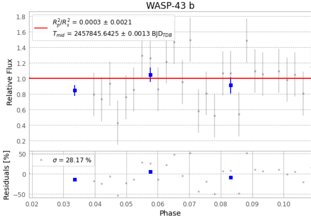
Figure 1 — FinalLightCurve_WASP-43 b_2017-04-01.png (SHA-256 7dfbff6bb507362a...)
