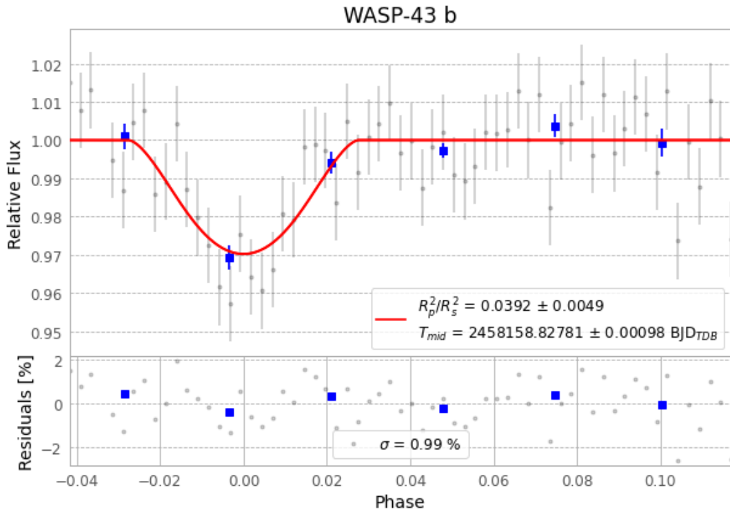
Figure 1 — FinalLightCurve_WASP-43 b_2018-02-08.png (SHA-256 6df82dda72acb27a...)
