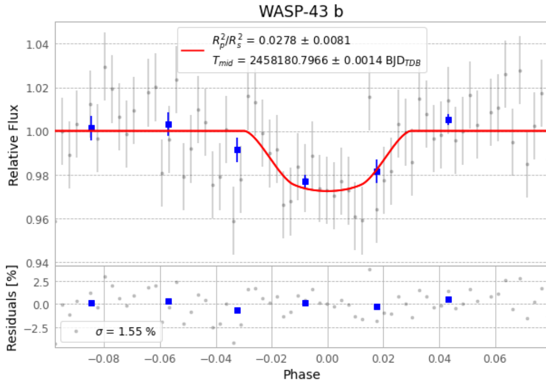
Figure 1 — FinalLightCurve_WASP-43 b_2018-03-02.png (SHA-256 545ddc43daa7afa3...)
