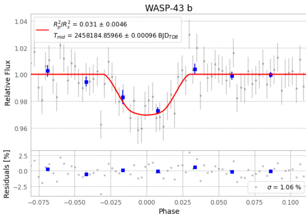
Figure 1 — FinalLightCurve_WASP-43 b_2018-03-06.png (SHA-256 4fa4b23ba09ded6e...)
