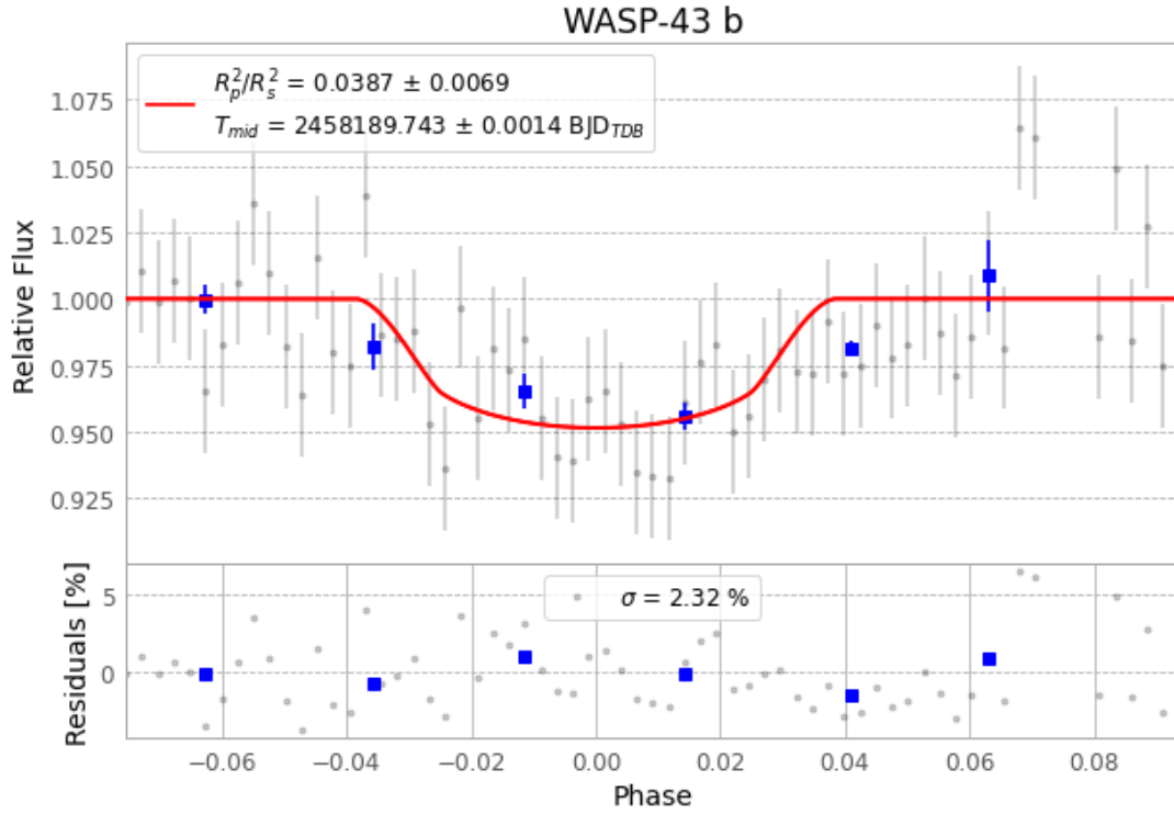
Figure 1 — FinalLightCurve_WASP-43 b_2018-03-11.png (SHA-256 82aaf823cd8d601b...)
