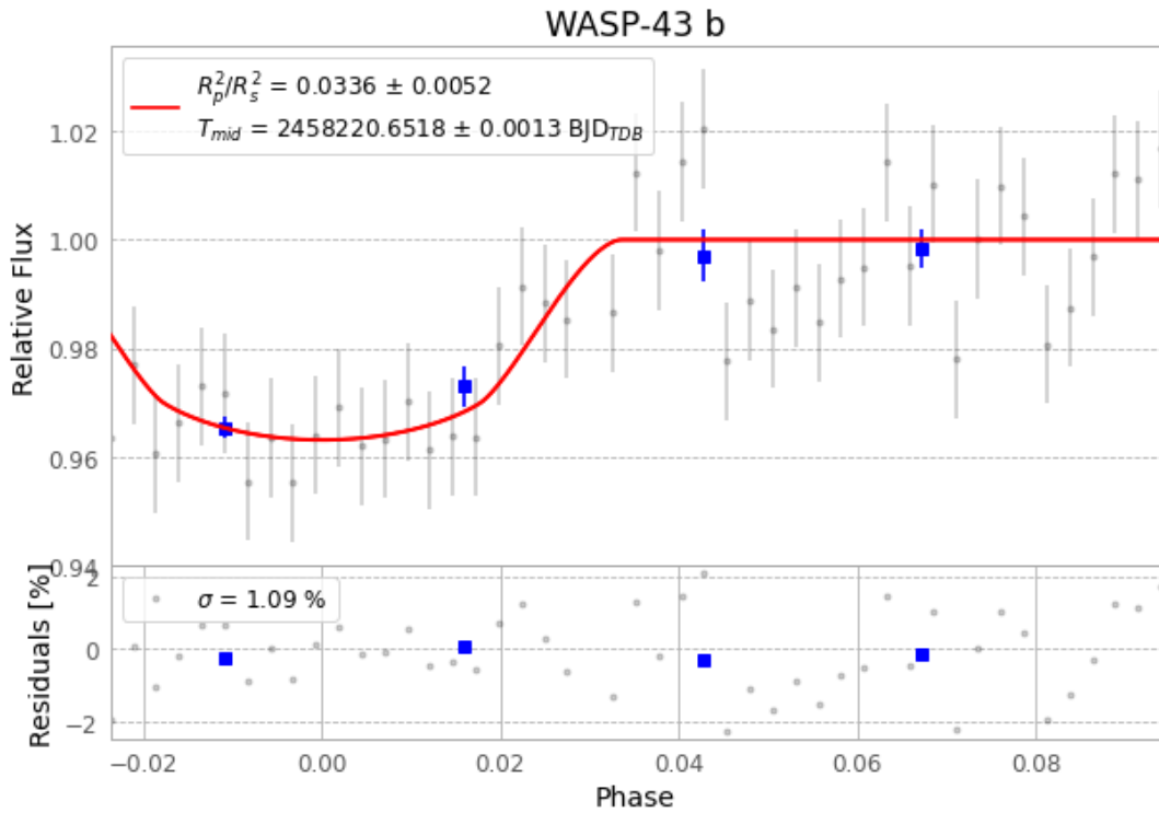
Figure 1 — FinalLightCurve_WASP-43 b_2018-04-11.png (SHA-256 37afb665fc2407dd...)
