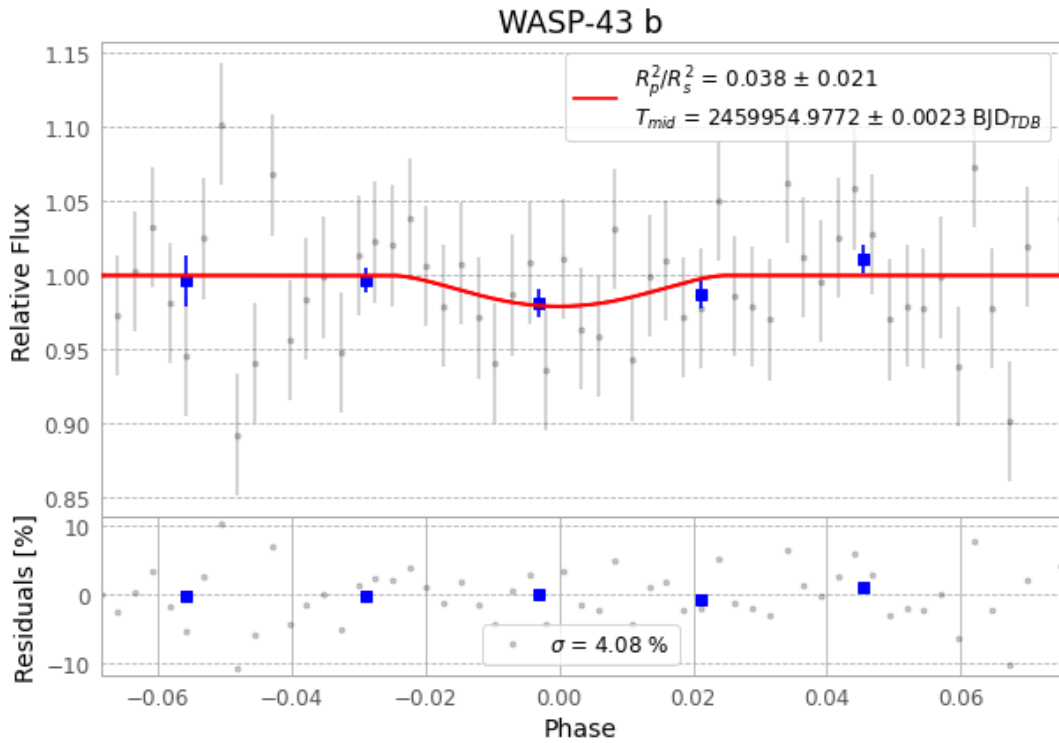
Figure 1 — FinalLightCurve_WASP-43 b_2023-01-10.png (SHA-256 514eca5112930346...)
