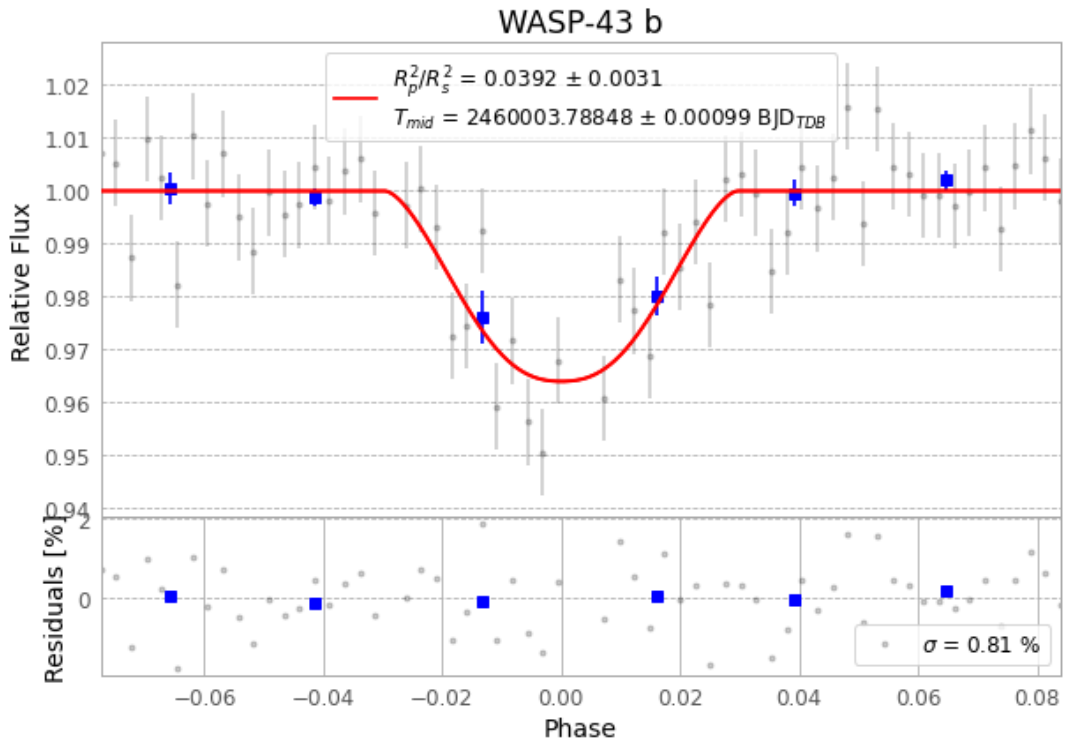
Figure 1 — FinalLightCurve_WASP-43 b_2023-02-27.png (SHA-256 cb1ac20dc9de094e...)
