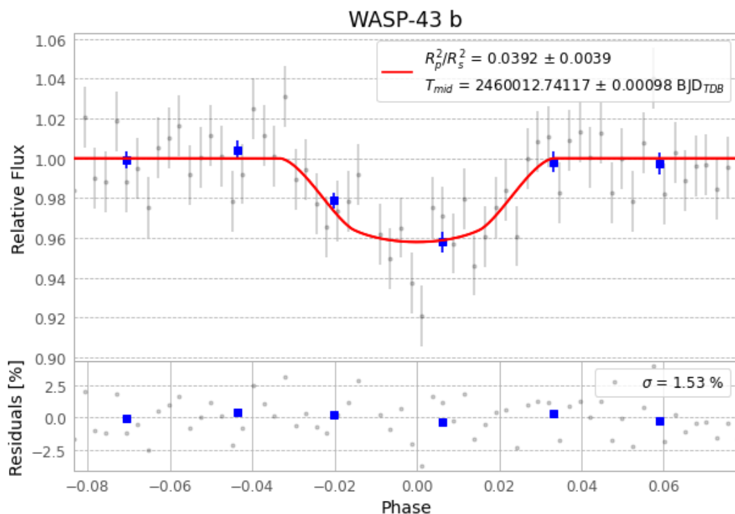
Figure 1 — FinalLightCurve_WASP-43 b_2023-03-08.png (SHA-256 03cf113f2e6c940a...)
