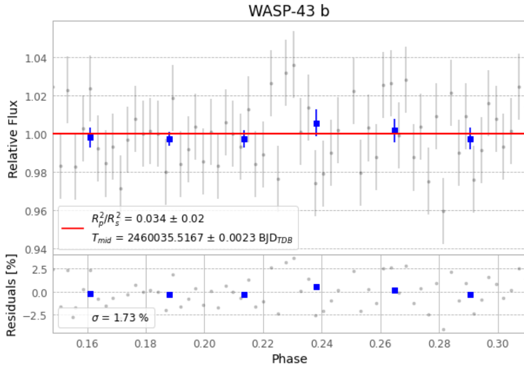
Figure 1 — FinalLightCurve_WASP-43 b_2023-03-31.png (SHA-256 2fd1bb26fe9b6176...)
