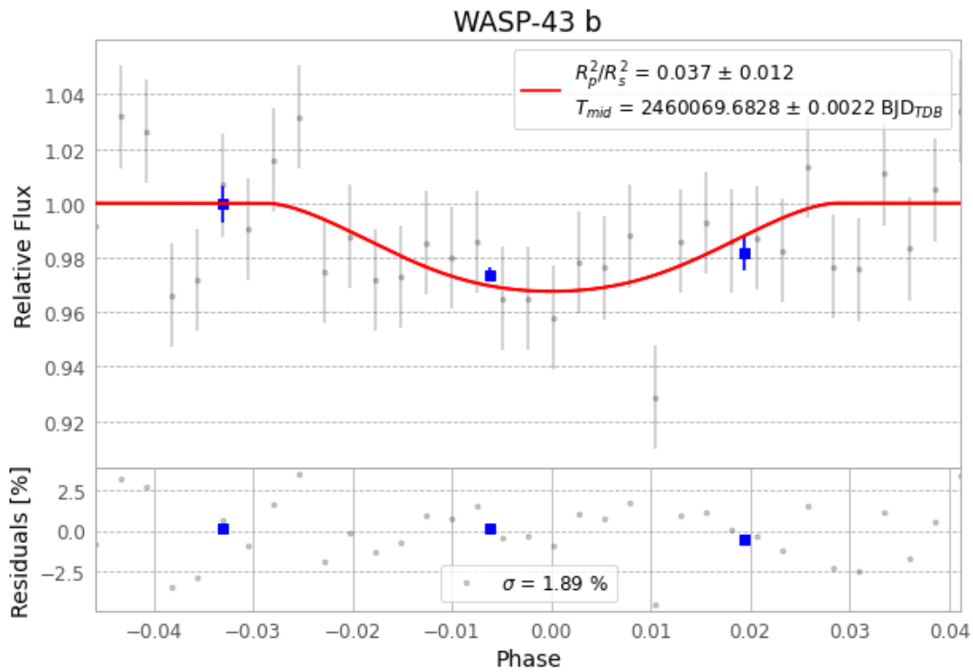
Figure 1 — FinalLightCurve_WASP-43 b_2023-05-04.png (SHA-256 2106198efc049c89...)
