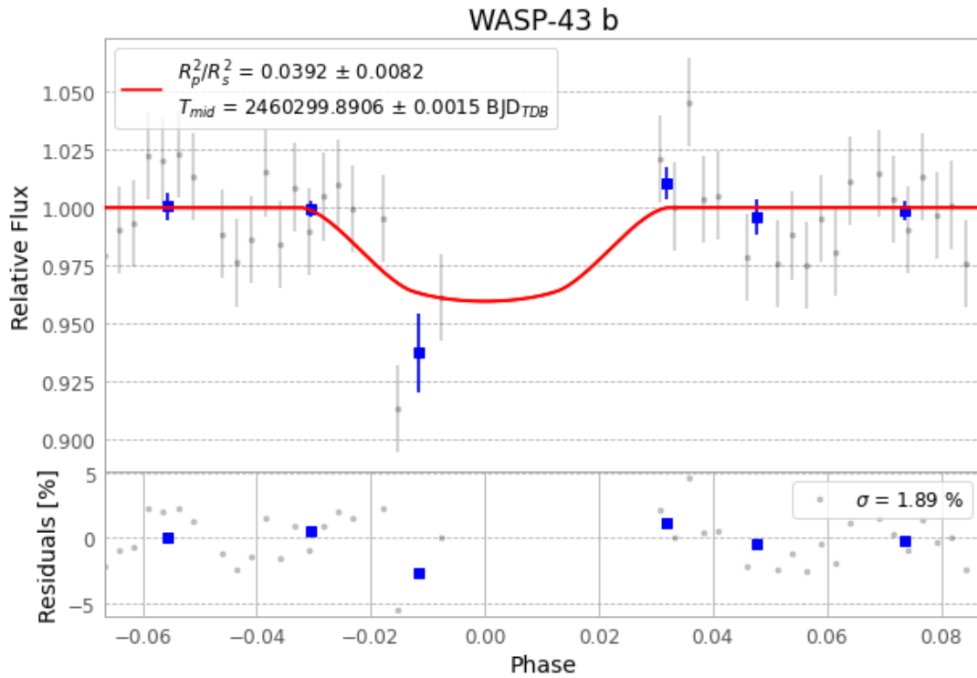
Figure 1 — FinalLightCurve_WASP-43 b_2023-12-21.png (SHA-256 93a768cca025b341...)
