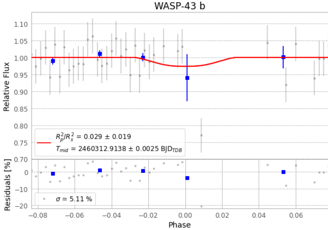
Figure 1 — FinalLightCurve_WASP-43 b_2024-01-03.png (SHA-256 1cd9a67b3a0b87b0...)
