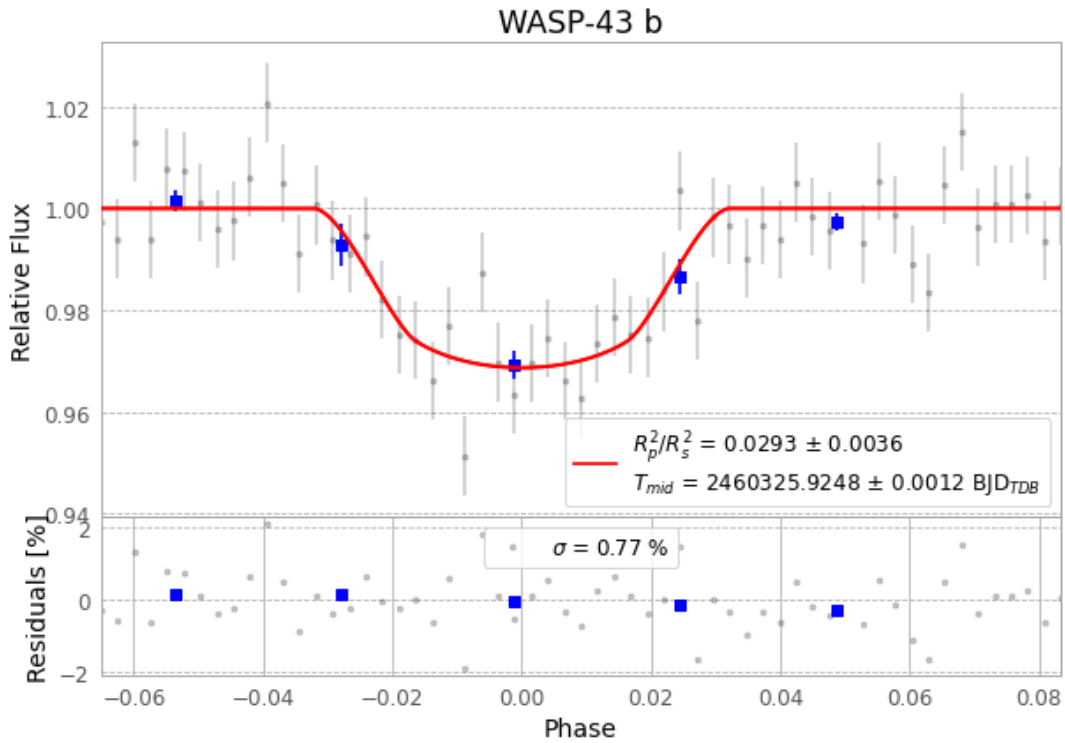
Figure 1 — FinalLightCurve_WASP-43 b_2024-01-16.png (SHA-256 efe3108f45ce0292...)
