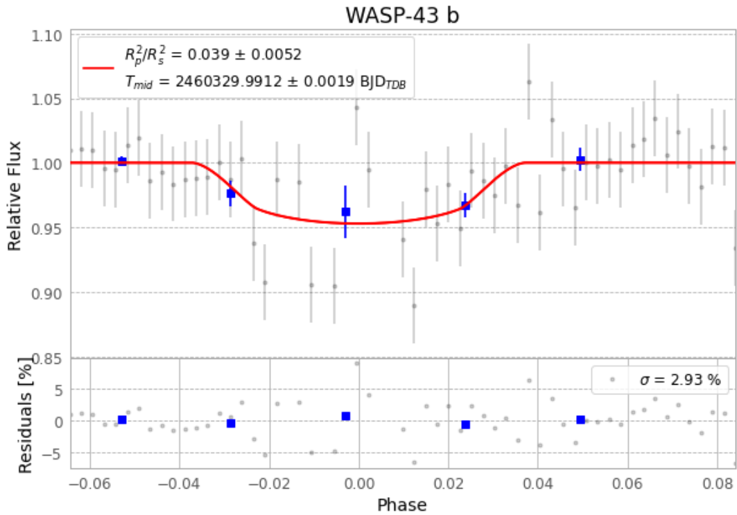
Figure 1 — FinalLightCurve_WASP-43 b_2024-01-20.png (SHA-256 cc6451753ed8cb9c...)
