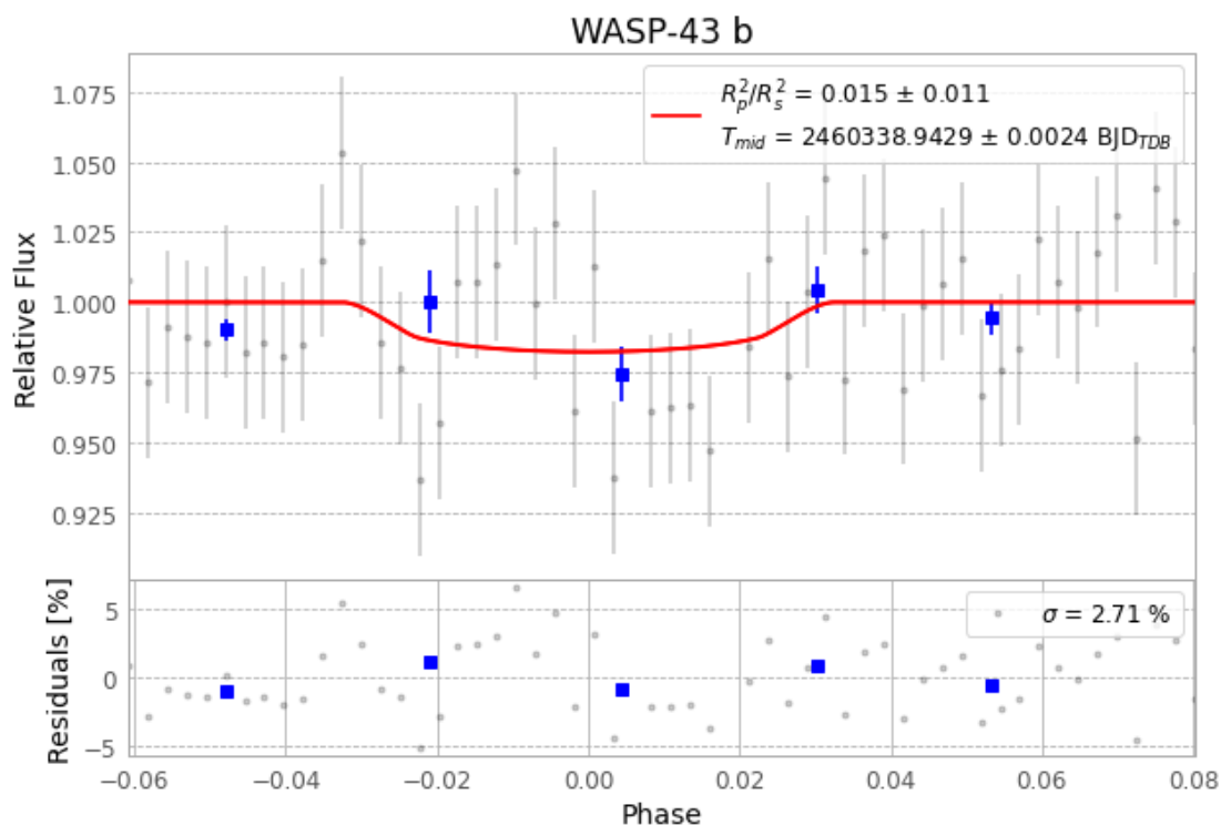
Figure 1 — FinalLightCurve_WASP-43 b_2024-01-29.png (SHA-256 729a7d5e7e5d1197...)
