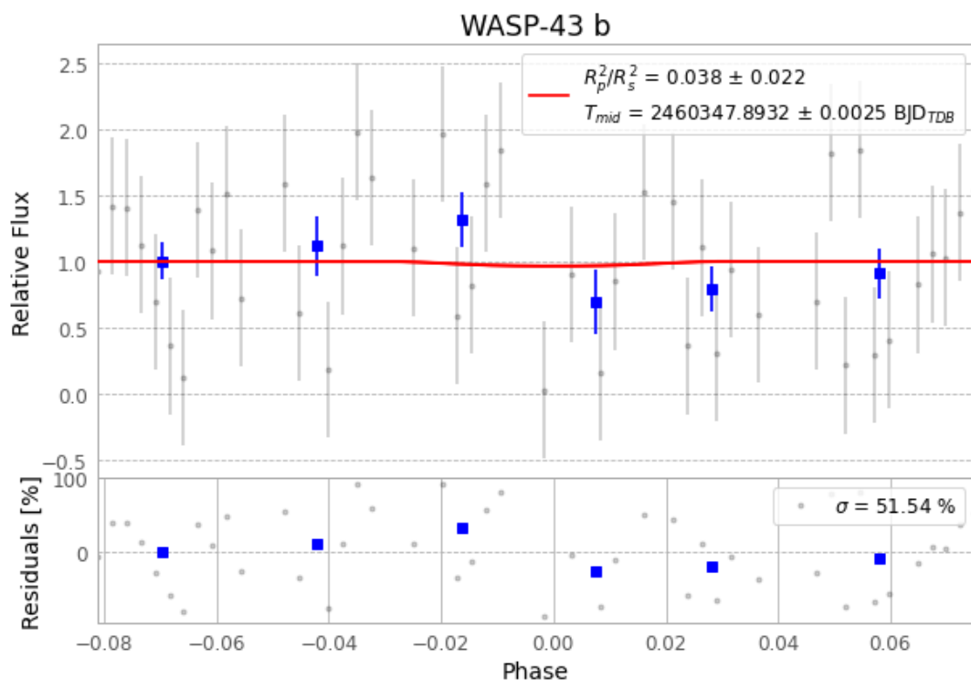
Figure 1 — FinalLightCurve_WASP-43 b_2024-02-07.png (SHA-256 6e906b701b00df38...)
