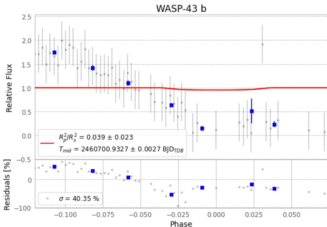
Figure 1 — FinalLightCurve_WASP-43 b_2025-01-25.png (SHA-256 05c03c4857666baa...)
