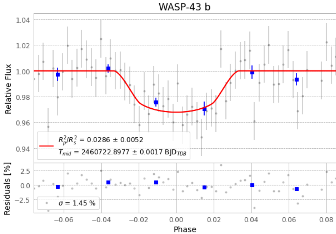
Figure 1 — FinalLightCurve_WASP-43 b_2025-02-16.png (SHA-256 68c8aaa3aa5a2273...)
