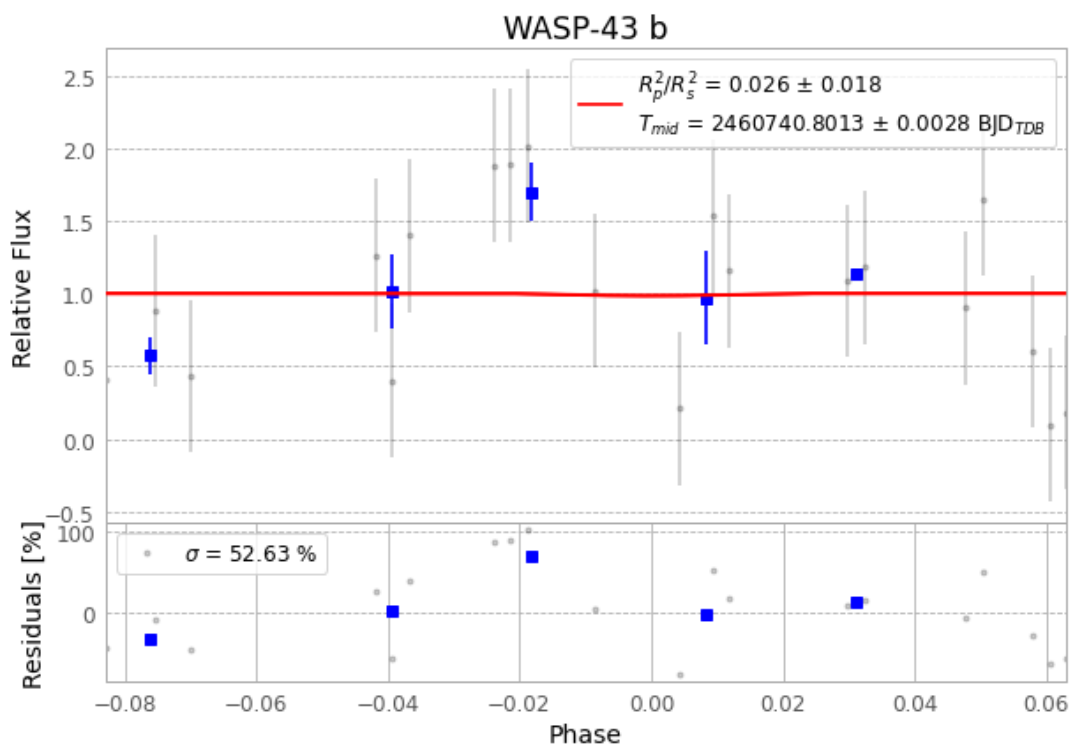
Figure 1 — FinalLightCurve_WASP-43 b_2025-03-05.png (SHA-256 e1c56ea8d6dca8cf...)
