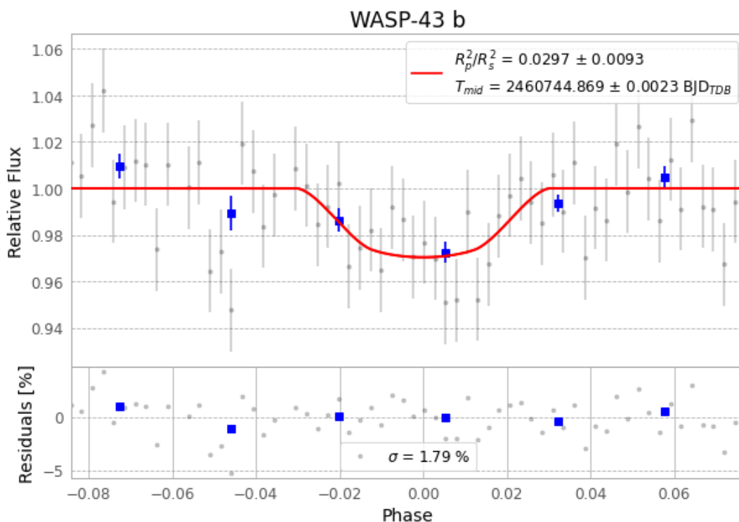
Figure 1 — FinalLightCurve_WASP-43 b_2025-03-10.png (SHA-256 e7015e58f572d32a...)
