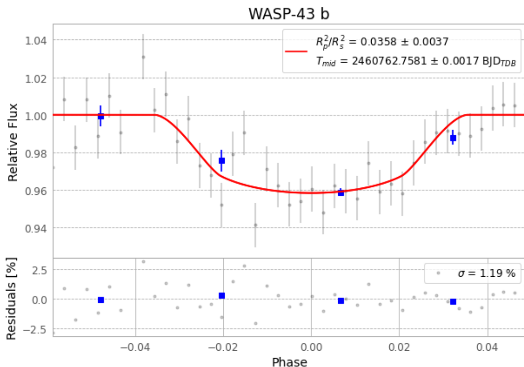
Figure 1 — FinalLightCurve_WASP-43 b_2025-03-27.png (SHA-256 3c411dea2025ad07...)
