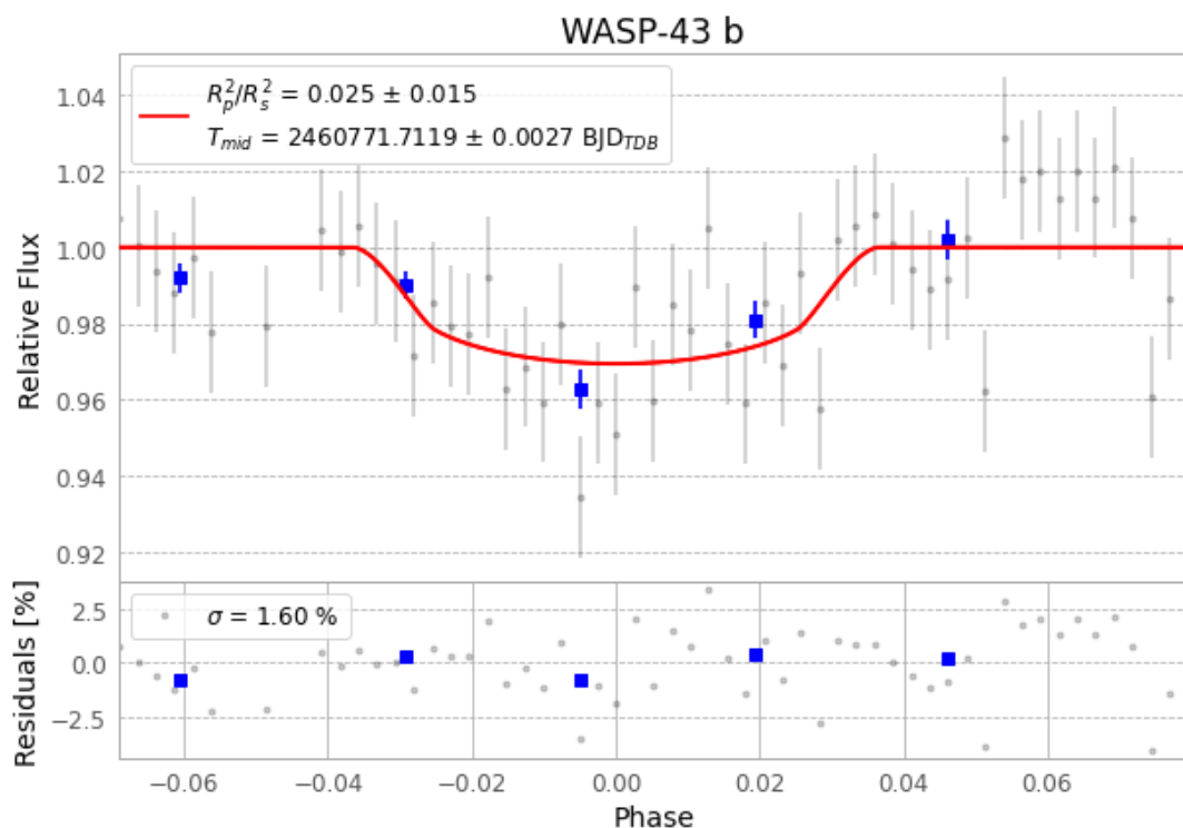
Figure 1 — FinalLightCurve_WASP-43 b_2025-04-05.png (SHA-256 54b5e84059e3933a...)
