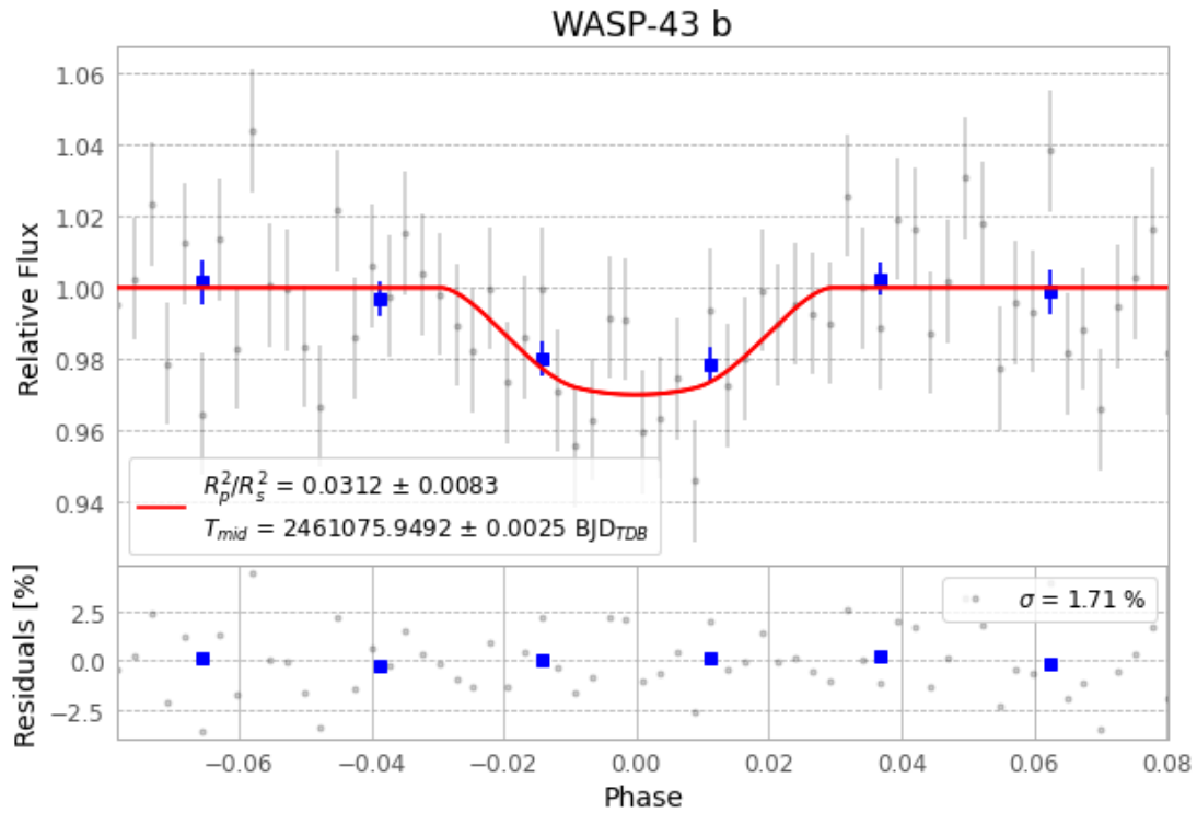
Figure 1 — FinalLightCurve_WASP-43 b_2026-02-04.png (SHA-256 927719cb53015436...)
